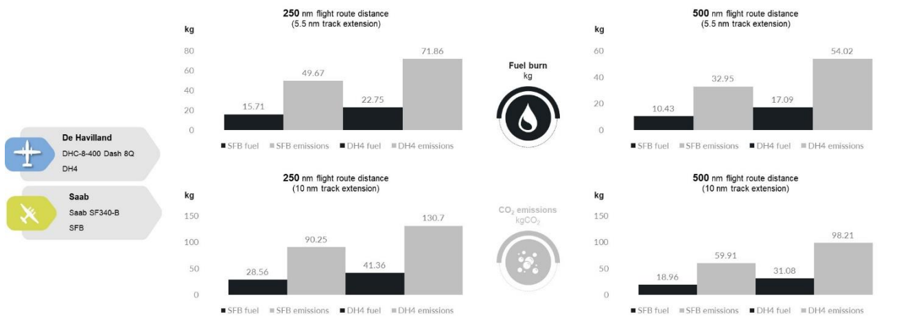
Figure 8.1 Fuel consumption and CO 2 emissions per movement for selected non-jet aircraft types
