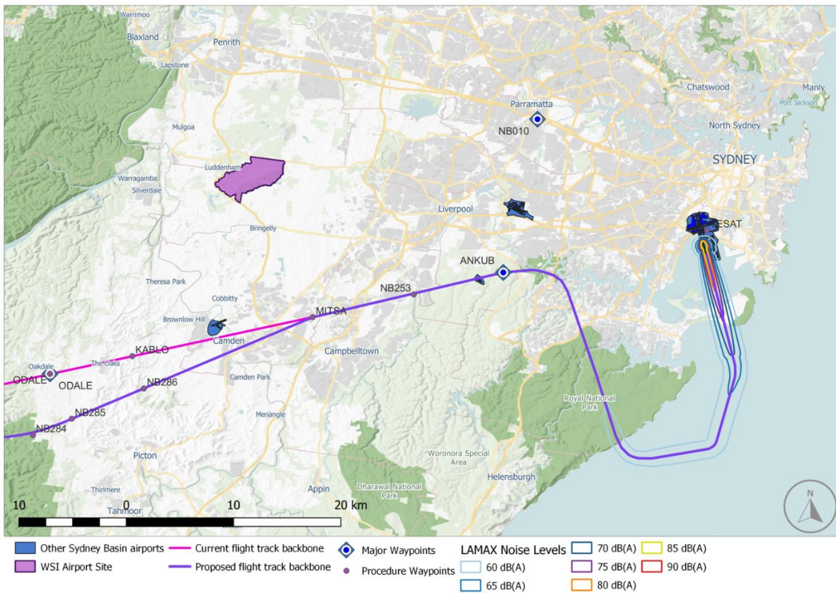
Figure 7.2 Proposed AKMIR STAR – L Am contours for an Airbus A330-300 arrival
