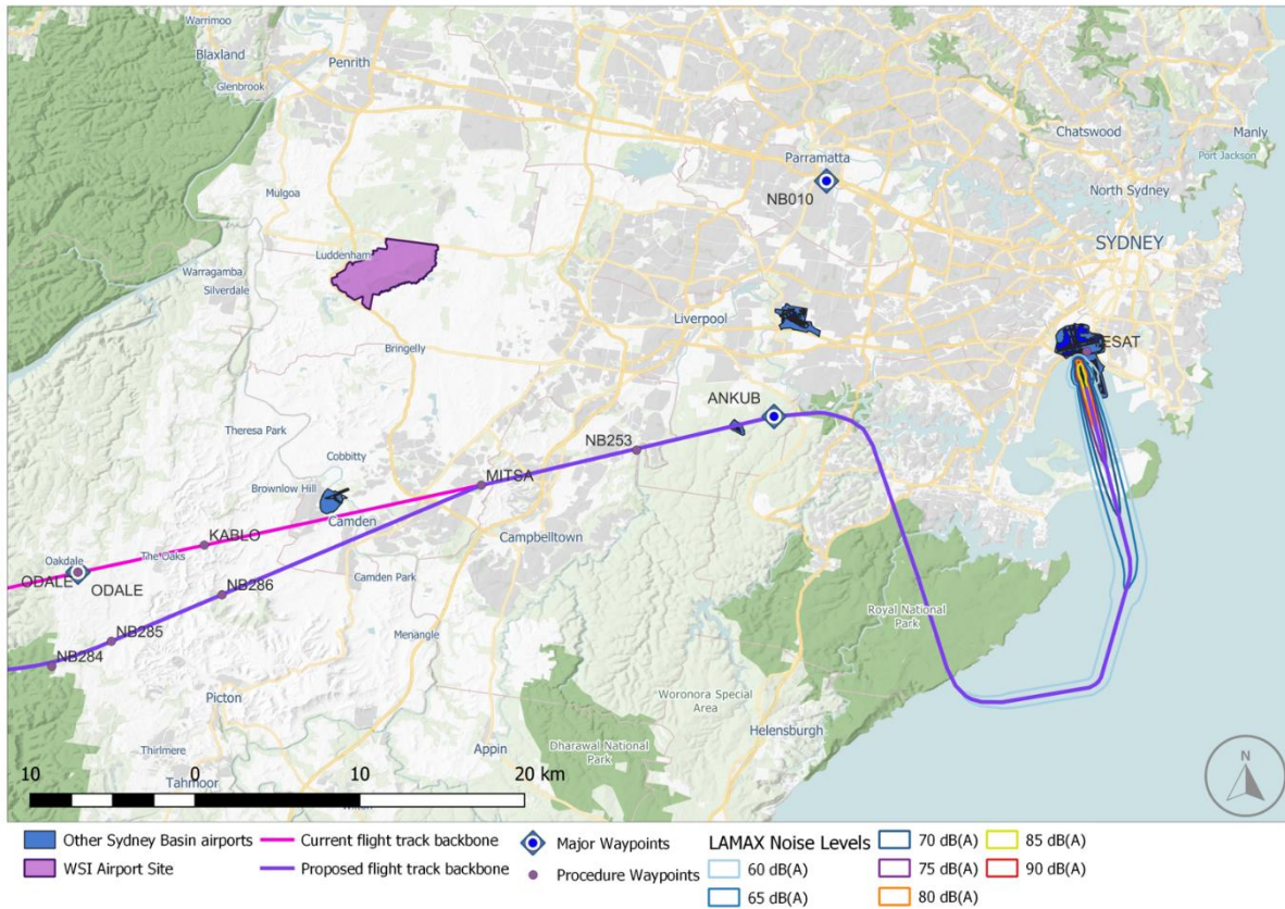
Figure 7.3 Proposed AKMIR STAR – L Amax contours for Boeing 737-800 arrival
